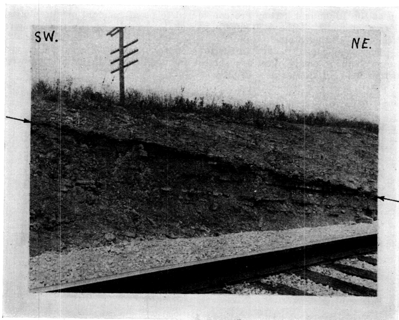
Fig. 1.—Looking north at the Ordovician-Silurian contact, four miles southwest of Joliet.
