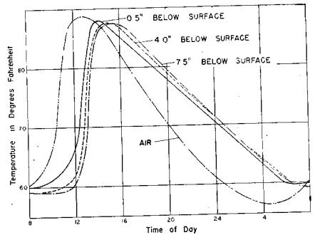
FIG. 3.—Typical temperature gradients in Class A evaporation pan.
