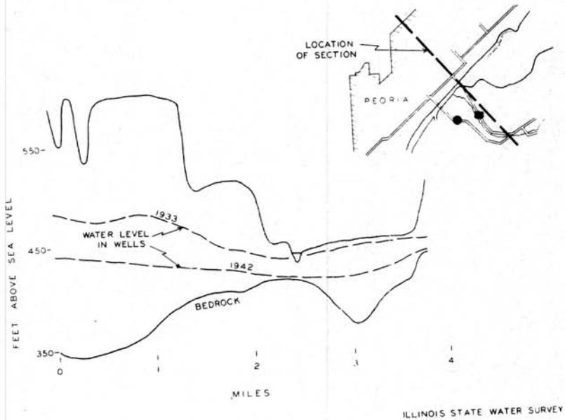
FIG. 7.—Groundwater cross-section at Peoria.
